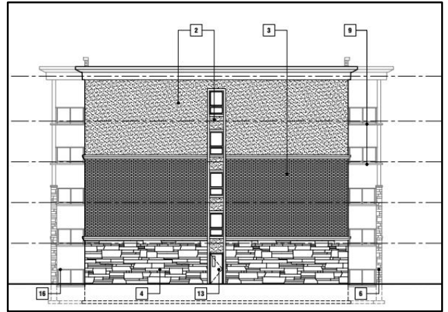
Side Elevation Facing Parking
