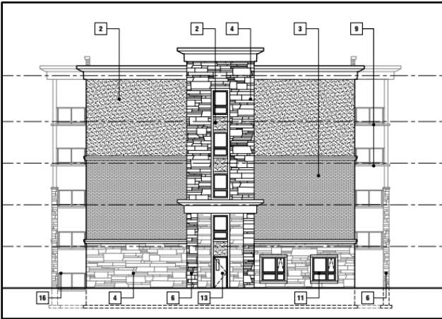
Side Elevation Facing Street
